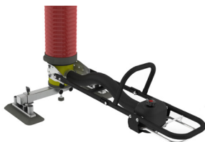
Flex handle with suction tool for side lifting
