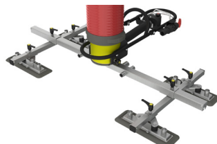
Flex handle with suction tool for side lifting
